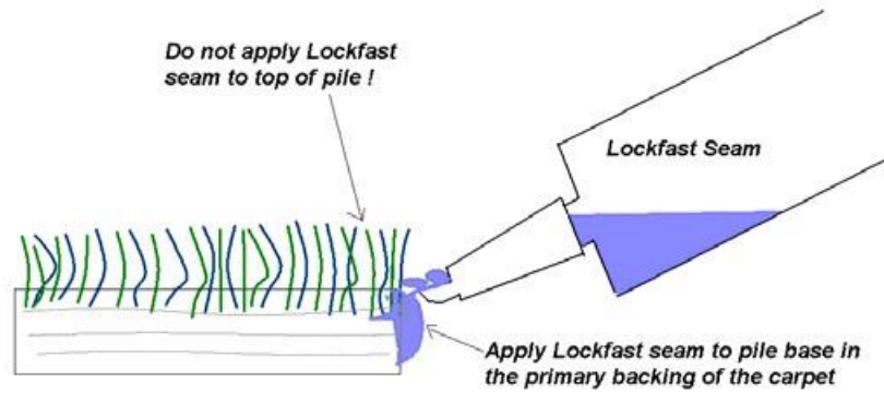
Correct Application of Lockfast Seam for tuft bonding in carpet
